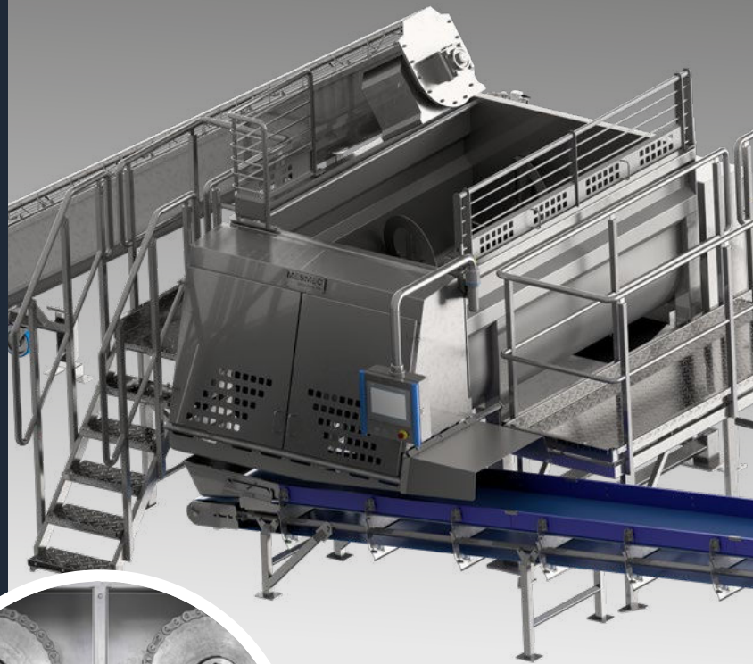
Mixing line solution with Mesmec OMX Mixer
